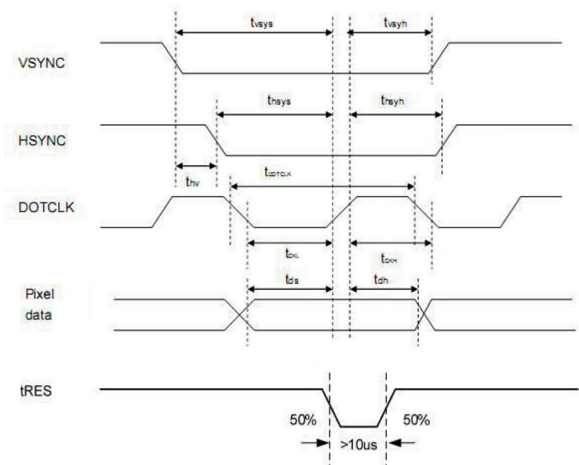
Figure 1: Pixel Timing
