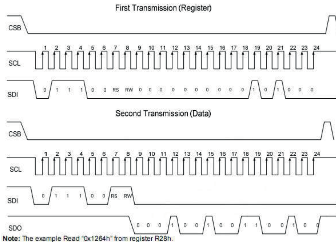
Figure 7:(b) SPI interface Timing Diagram &amp; Read SPI Example
